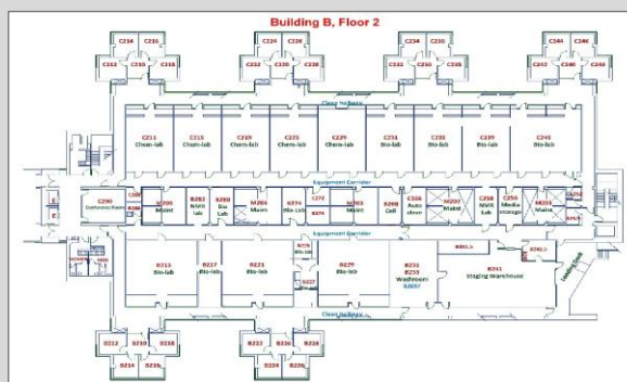
Layout – Office, R&D Lab
